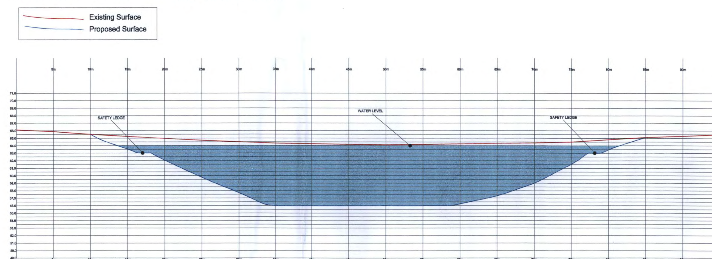
CROSS SECTION 1: PROPOSED DAM
